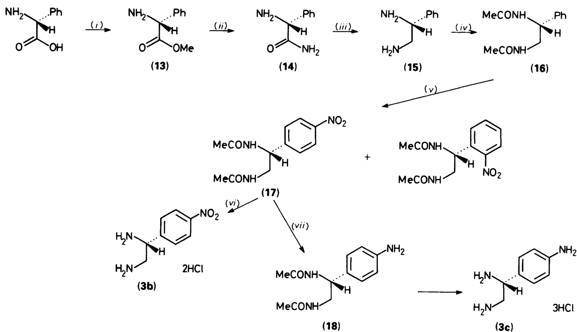
Scheme 3. (i) \text{SOCl}_2 , \text{MeOH} ; (ii) concentrated \text{NH}_3 ; (iii) \text{LiAlH}_4 ; (iv) (\text{MeCO})_2\text{O} ; (v) \text{HNO}_3 ; (vi) \text{HCl} , water; (vii) \text{H}_2 , \text{Pd-Al}_2\text{O}_3
