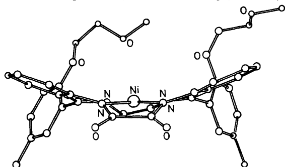
Figure 1. Perspective drawing of complex cis -(1a), derived from X-ray analysis data taken from ref. 7
