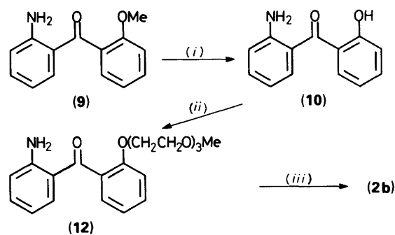
Scheme 2. (i) HBr, MeCO 2 H; (ii) tsO(CH 2 CH 2 O) 3 Me (11), K 2 CO 3 ; (iii) (COCl) 2
