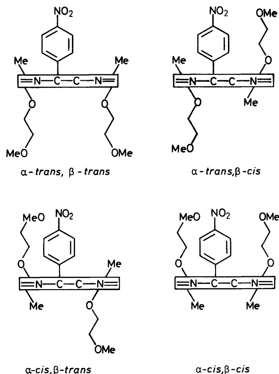
Figure 2. Schematic representation of the four isomers of complex (1b); cis and trans isomers are designated according to the relative orientation of the podands and the 4-nitrophenyl substituent
