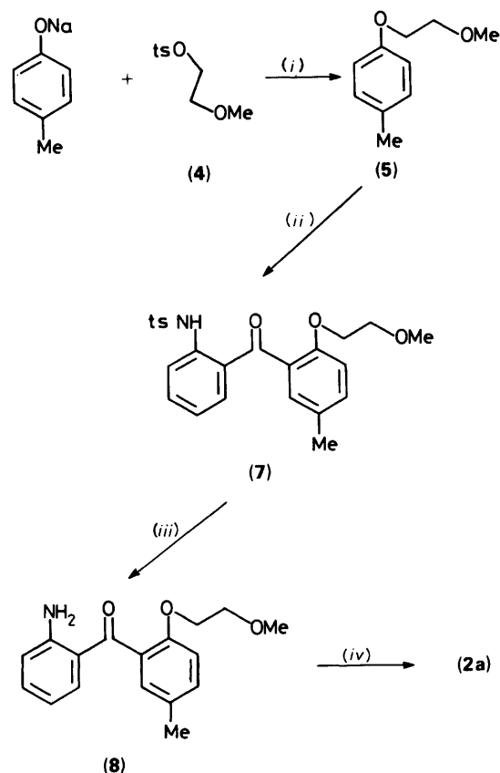
Scheme 1. ts = Tosyl. (i) MeOCH 2 CH 2 OH; (ii) compound (6), AlCl 3 ; (iii) H 2 SO 4 ; (iv) (COCl) 2
