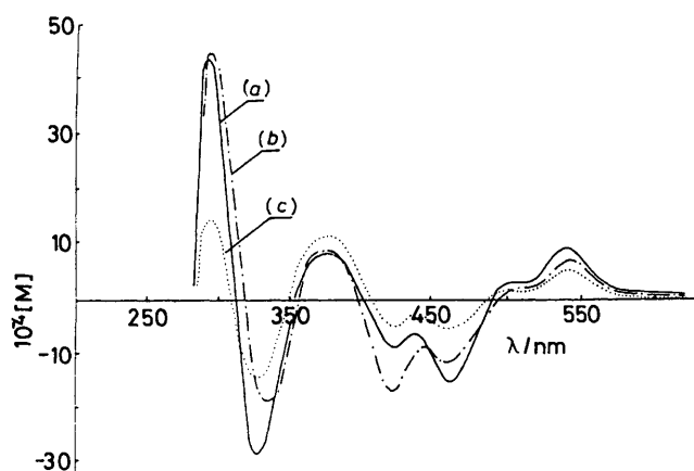
Figure 3. O.r.d. curves for individual isomers of complex (1b) in ethanol solution at 25 °C: (a) (I); (b) (II); and (c) (III)
